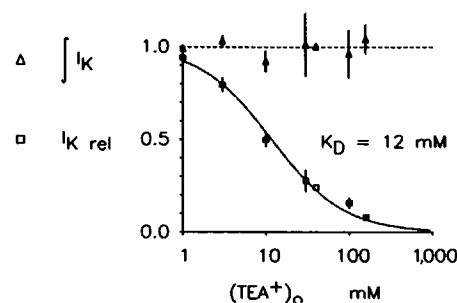
FIGURE 2 Effect of [TEA^+]_o on peak K^+ current amplitude, I_{K\text{ peak}} , and current integral I_K of the K^+ current. The TEA^+ dose-response curve on I_{K\text{ peak}} was determined as
