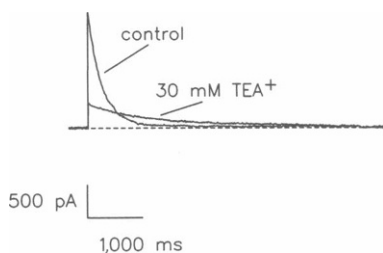
FIGURE 1 K^+ currents in a Jurkat cell in normal Ringer solution (control) and during application of a Ringer solution containing 30 mM TEA^+ . K^+ outward currents associated with 5-s depolarizing pulses to +40 mV from a holding potential of -80 mV. Cell 106.
